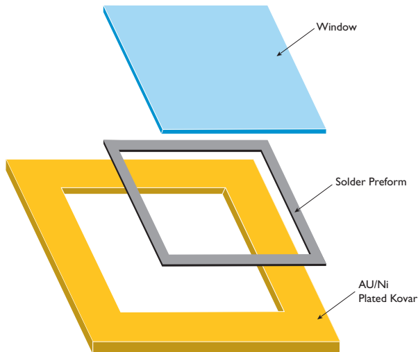
Glass inset on plated Kovar frame, configured for seam welding.
