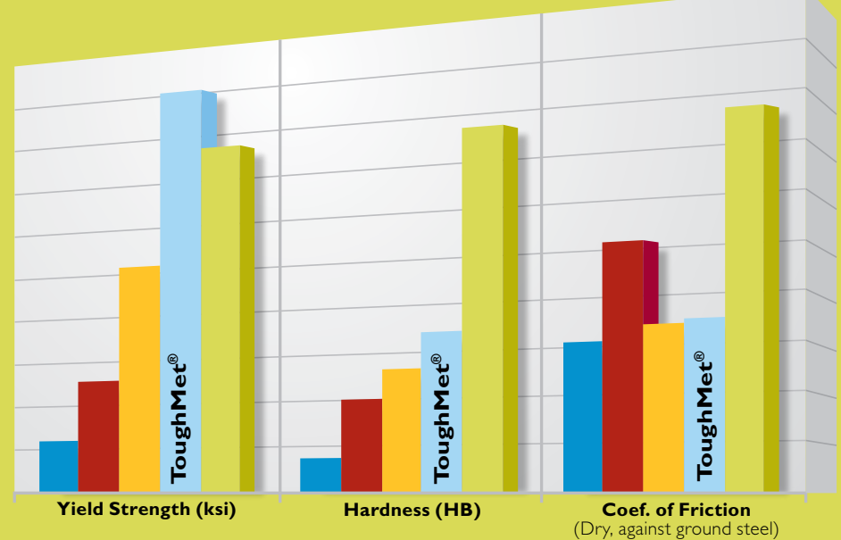
RELATIVE PROPERTIES OF BEARING MATERIALS
