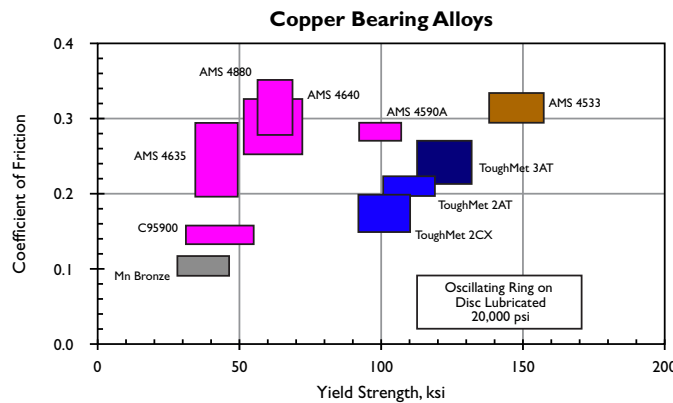
Figure 1. Friction Coefficient Measurement Results
