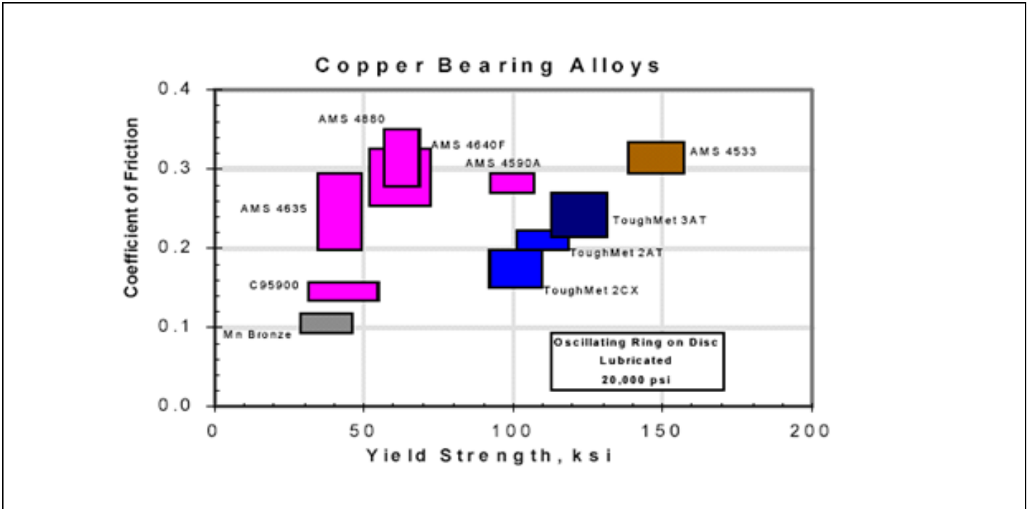
Figure 1. Friction Coefficient measurement results. Boxes represent spread in actual friction measurements and “typical” 0.2%
