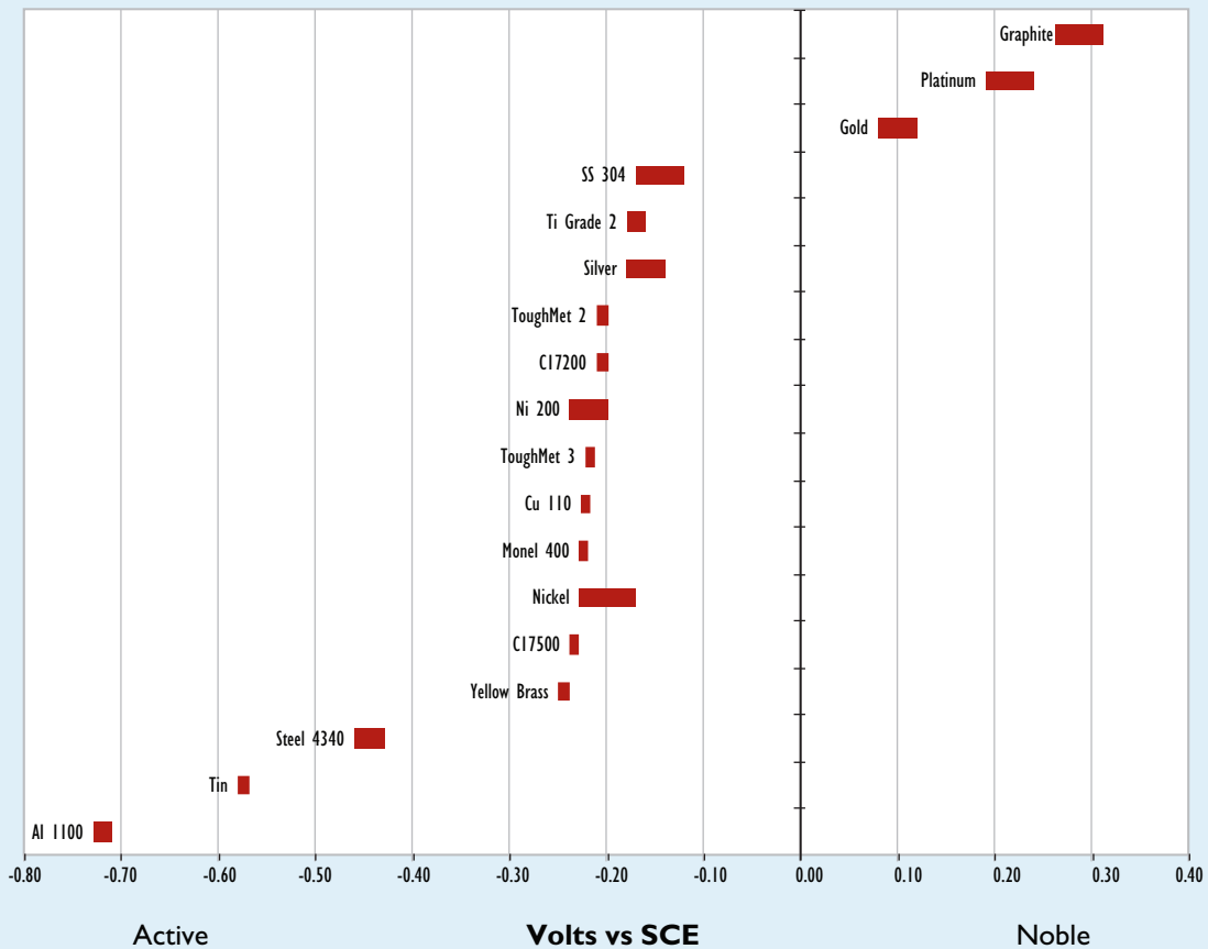
Galvanic Series in Simulated Seawater
