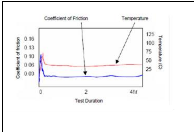
Figure 2: Thrust Bearing Test 2 Coefficient of Friction and Temperature
