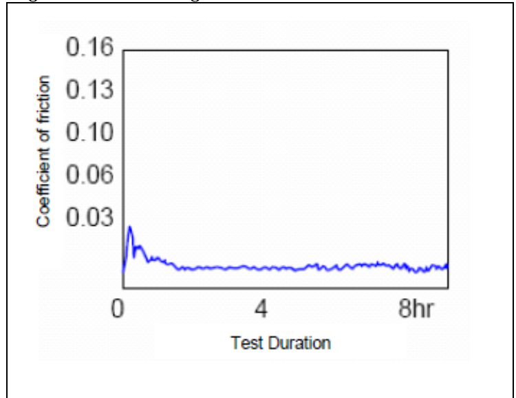
Figure 1: Thrust Bearing Test 1 Coefficient of Friction
