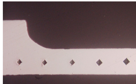
Electron Beam Zone Annealing (DPH indents show softening in bend location)
