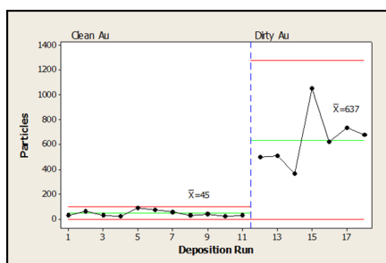
Reduced particle count associated with EVAPro® grade gold versus current industry standard.
